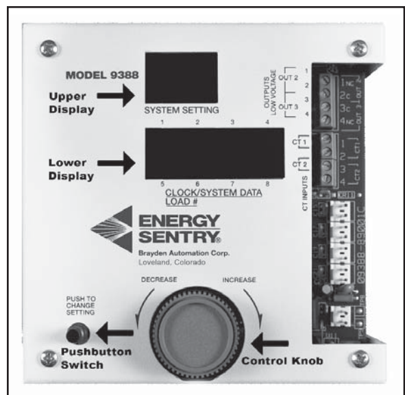
Figure 2. Control/Relay (C/R) Unit
