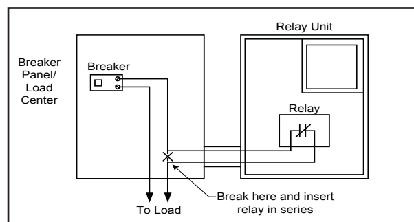
Figure 7. Power Relay Interconnection Schematic
